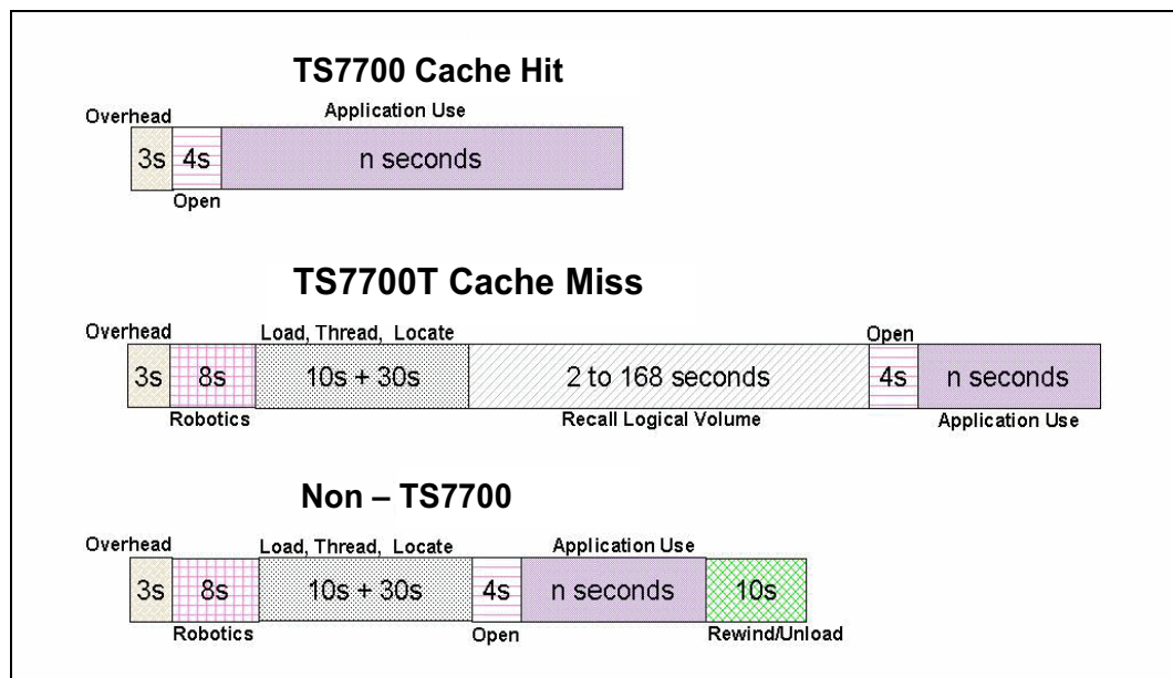
Figure 4-7 Tape processing time comparison example (not to scale)
